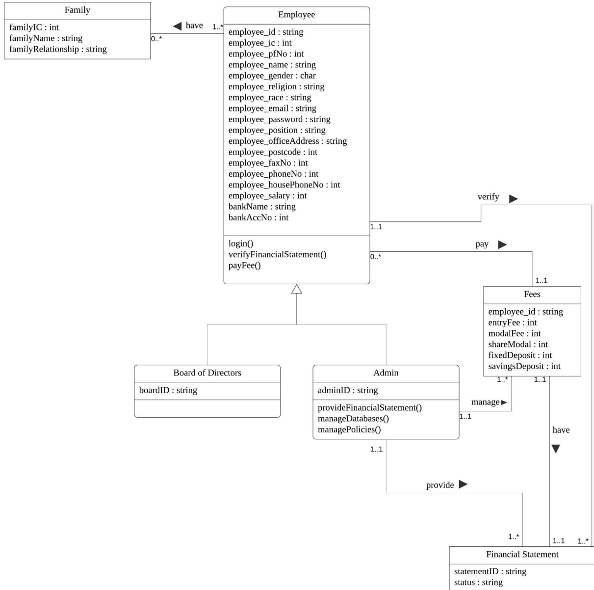
Figure 4.9: Class diagram for Financial Subsystem
