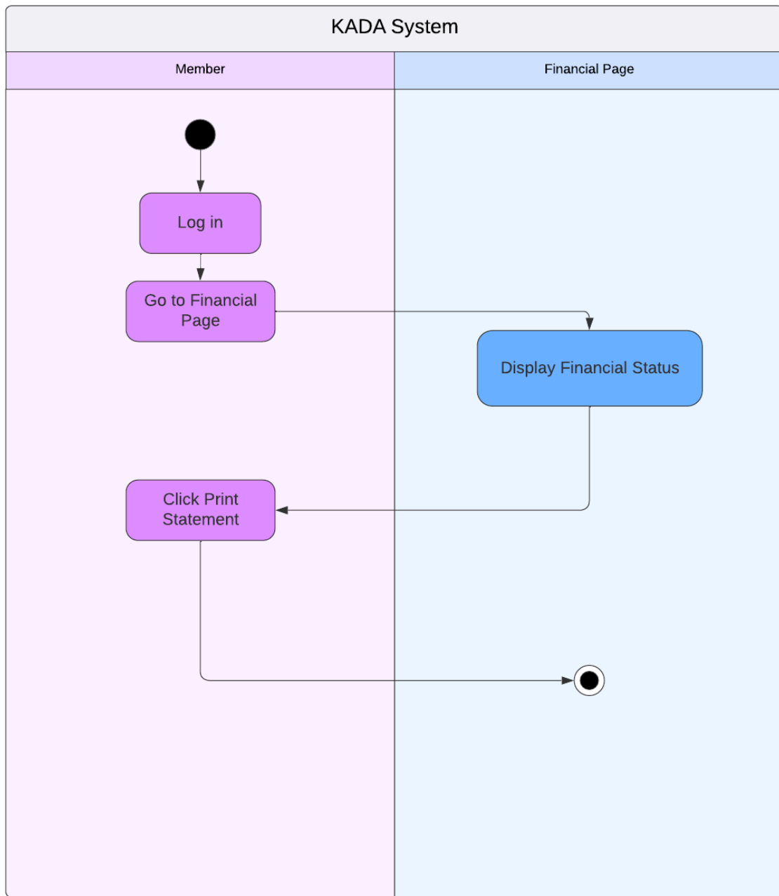
Figure 2.11: Activity Diagram for View Financial Statement
