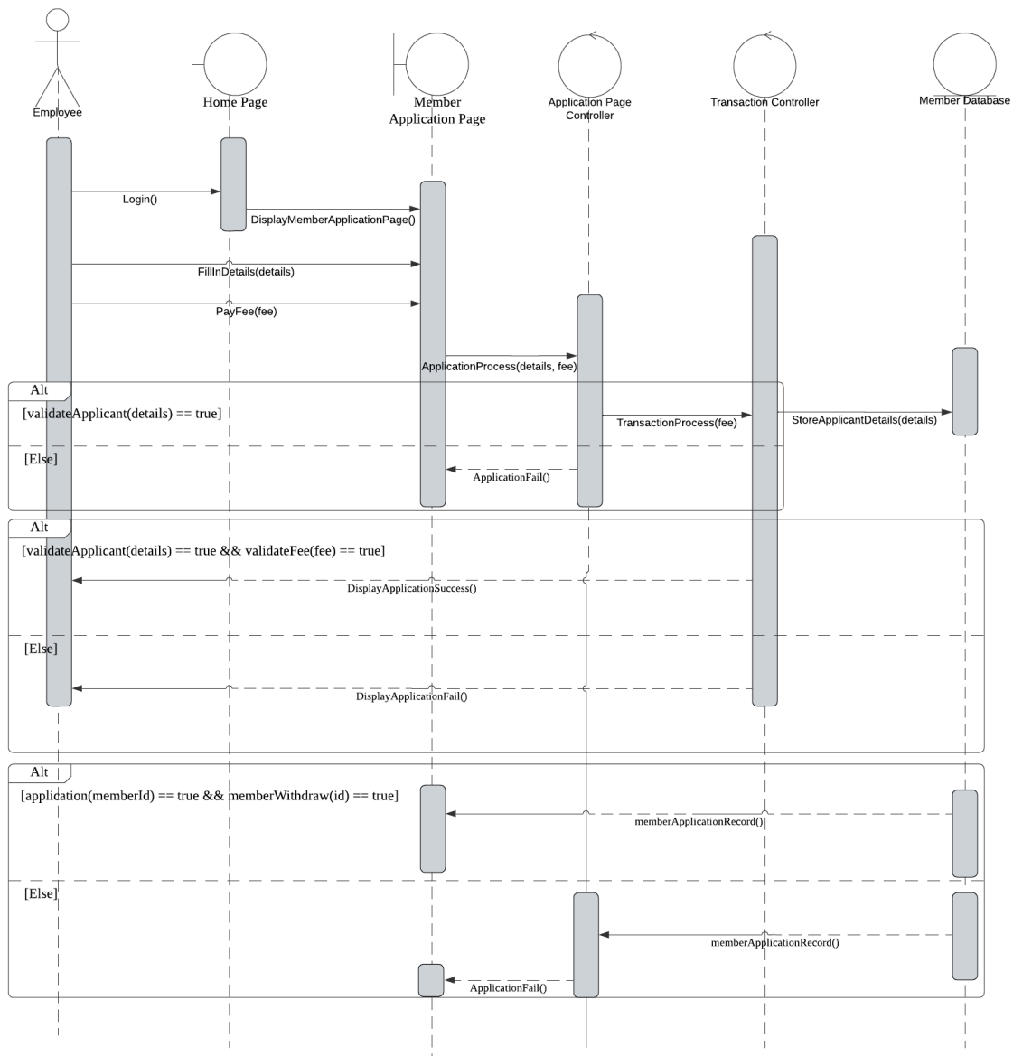
Figure 2.2: Sequence Diagram for Apply for Membership
