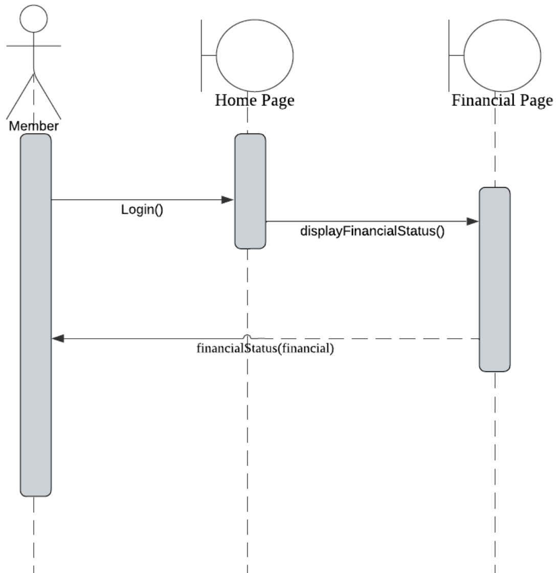
Figure 2.10: Sequence Diagram for View Financial Statement
