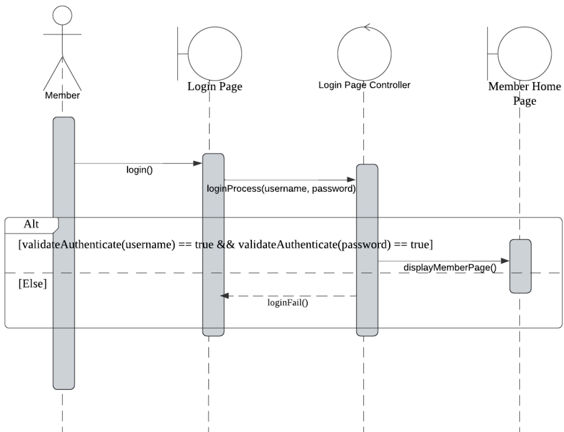
Figure 2.24: Sequence Diagram for Authentication (Member)
