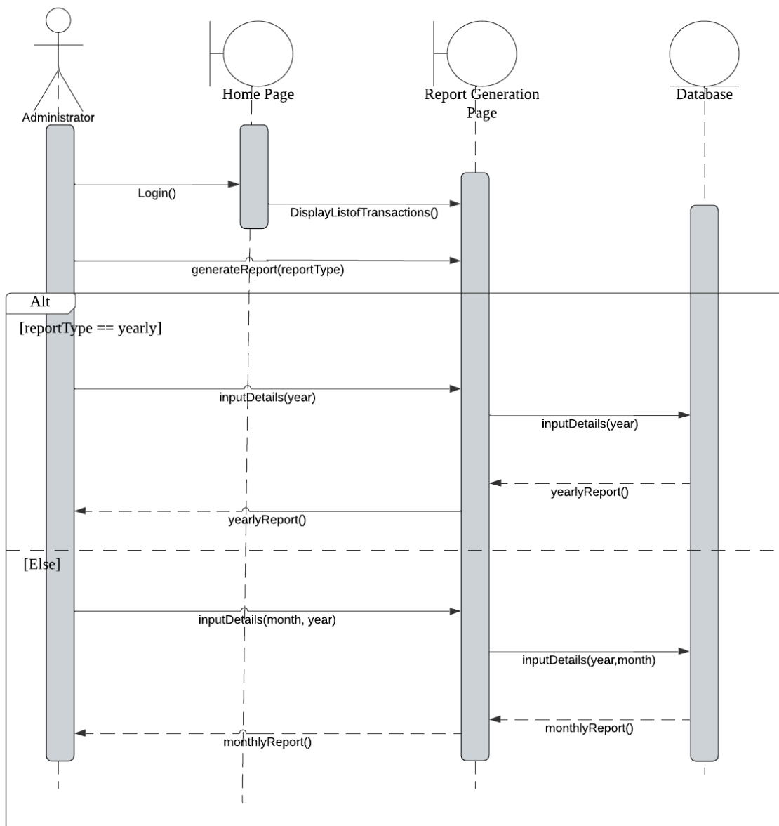
Figure 2.22: Sequence Diagram for Generate Report
