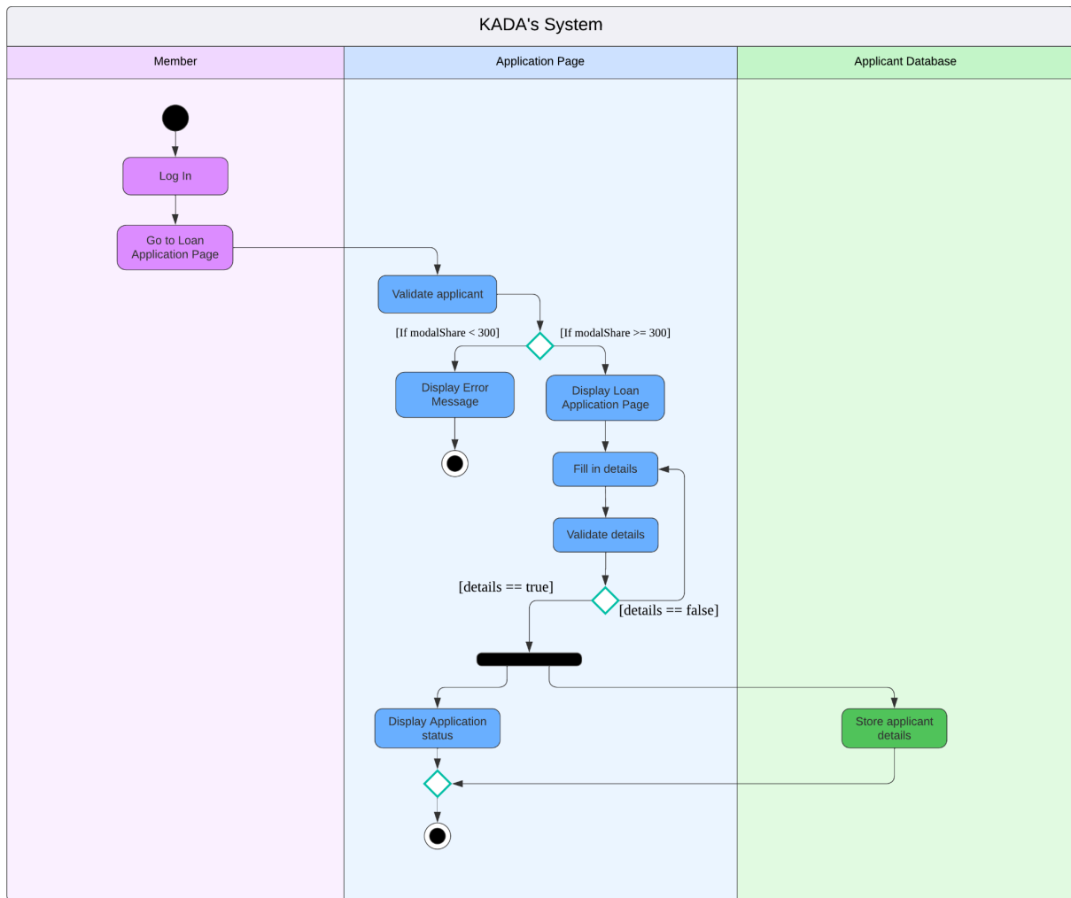
Figure 2.5: Activity Diagram for Apply for Loan
