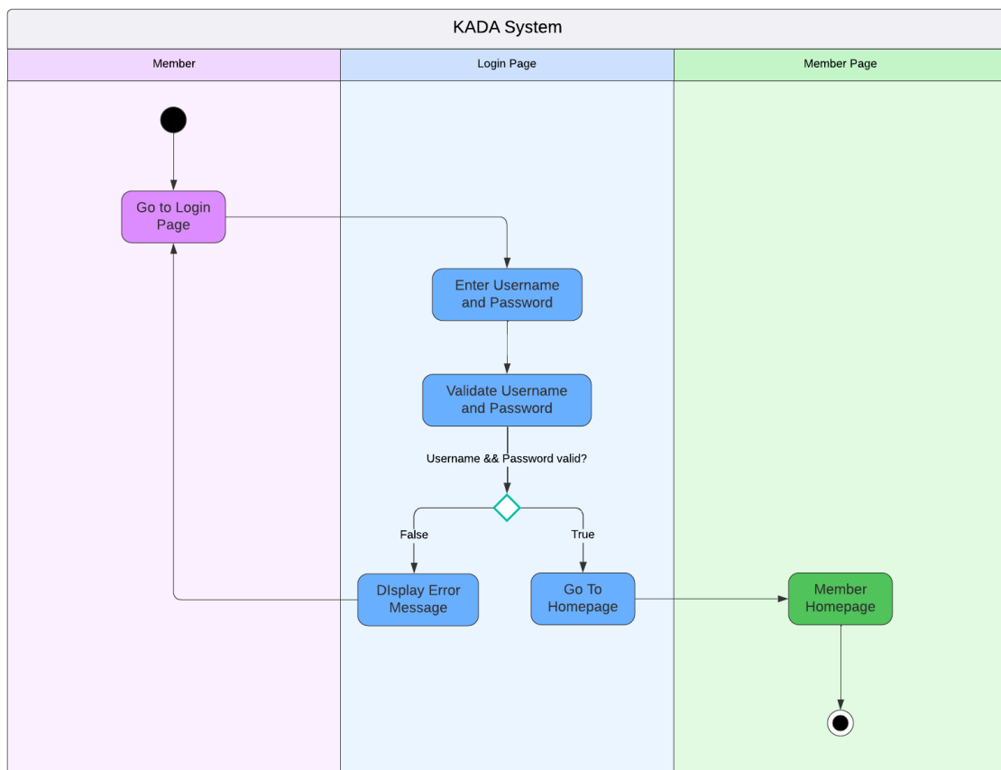
Figure 2.27: Activity Diagram for Authentication (Member)
