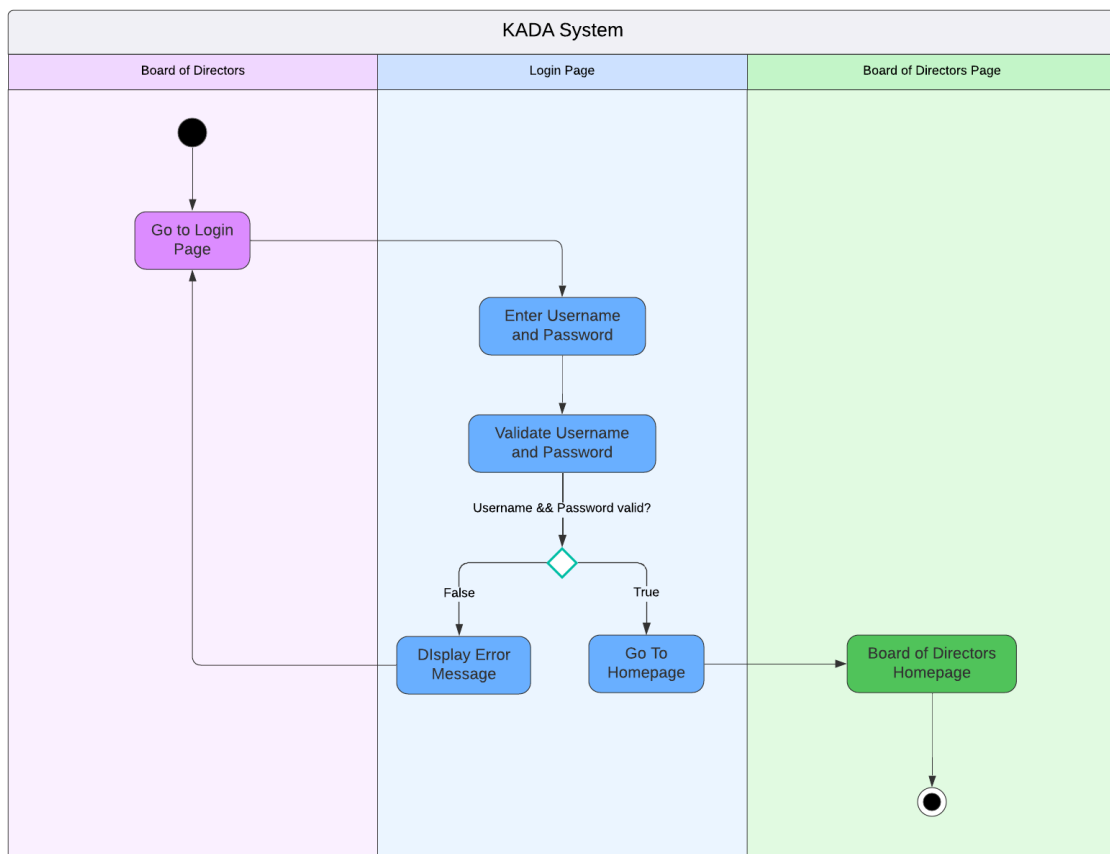
Figure 2.29: Activity Diagram for Authentication (Board of Directors)
