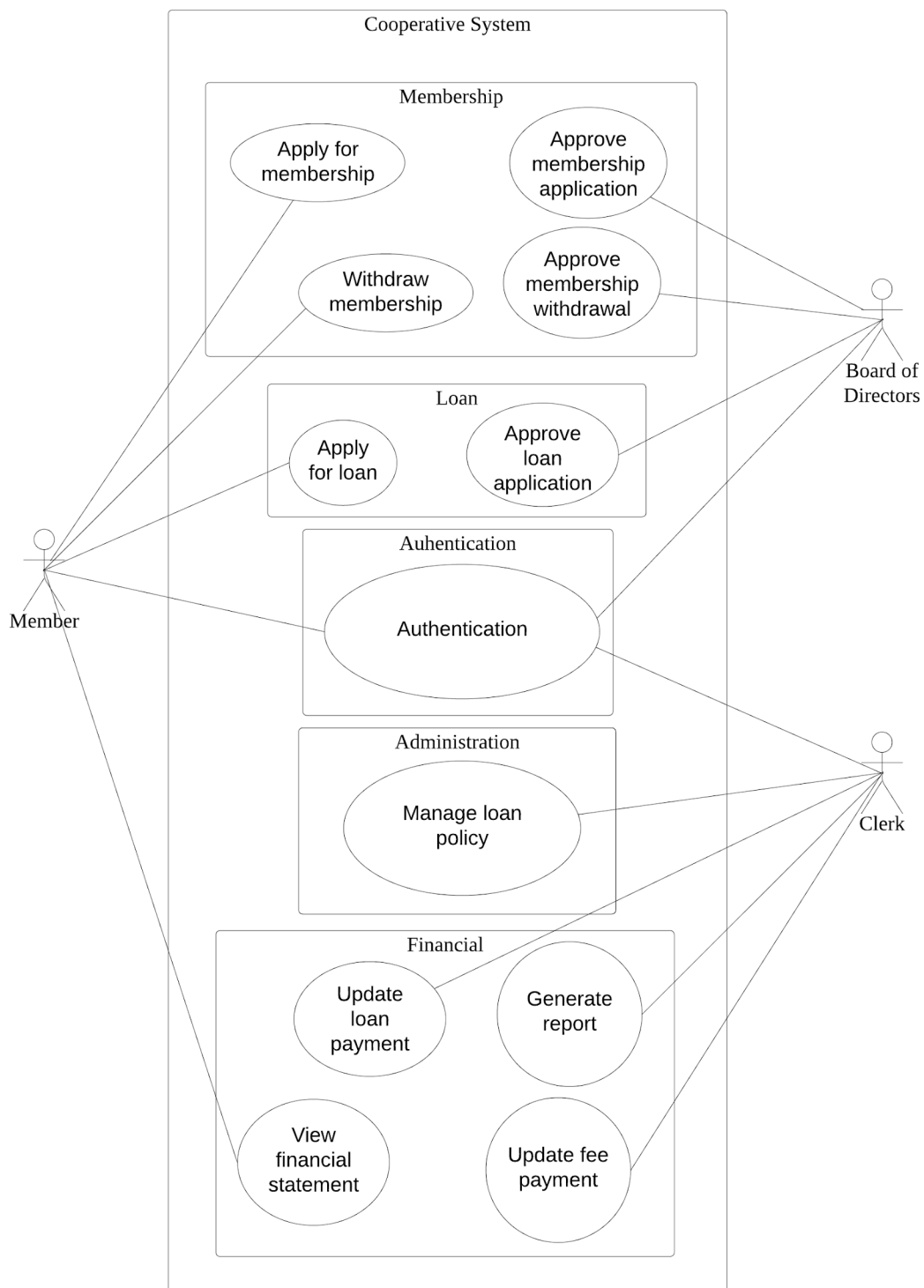
Figure 2.1: Use Case Diagram for KADA's Cooperative Web-Based System
