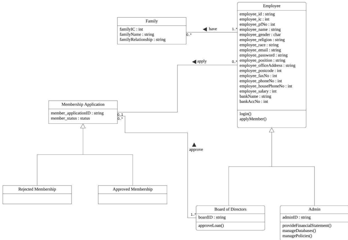
Figure 4.10: Class Diagram for Membership Subsystem
