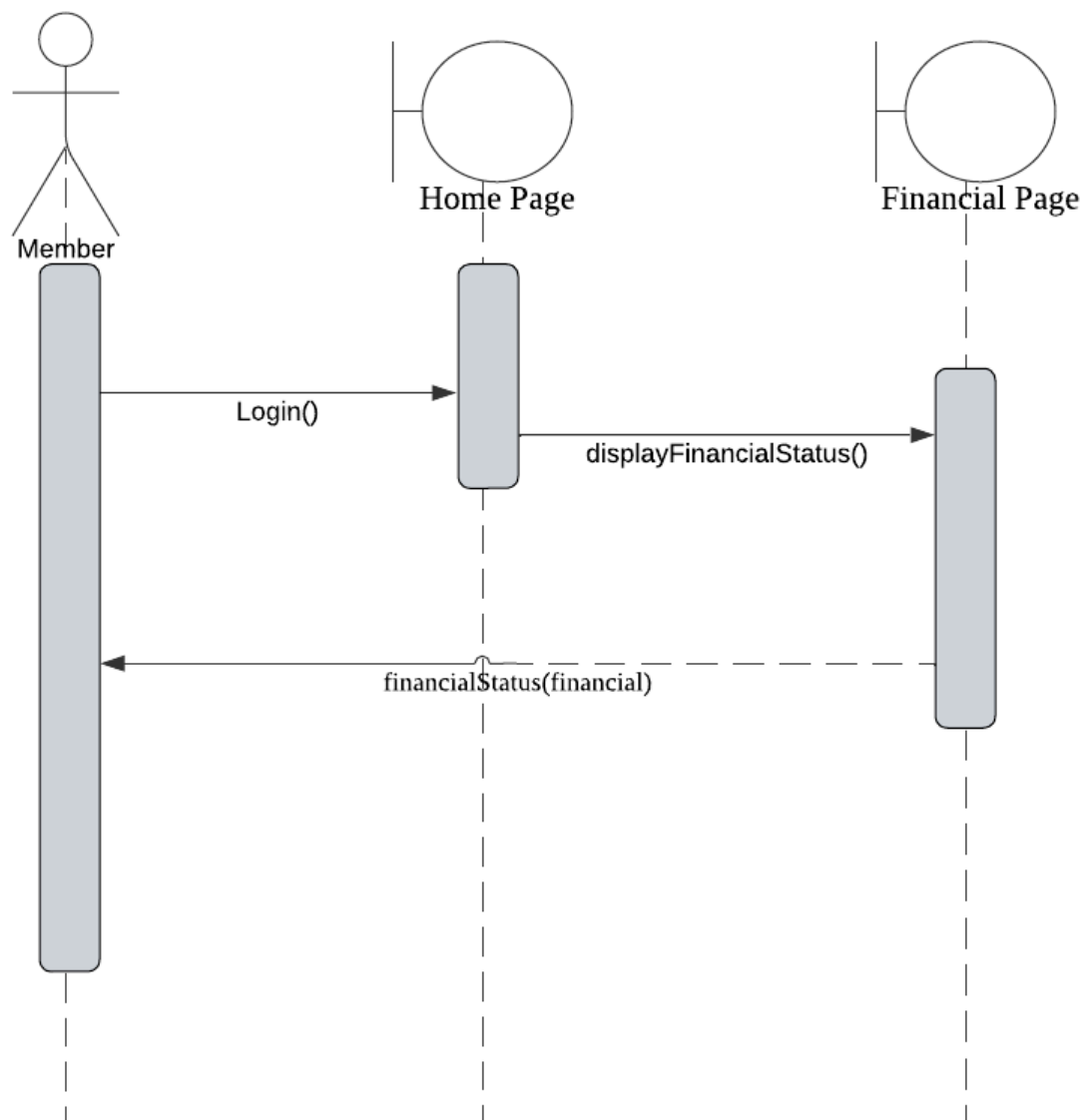
Figure 4.17: Sequence Diagram for View Financial Statement
