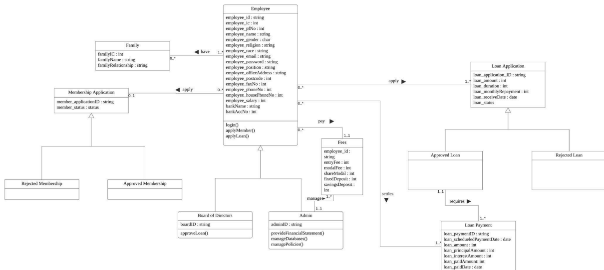
Figure 4.11 Class Diagram for Administration Subsystem
