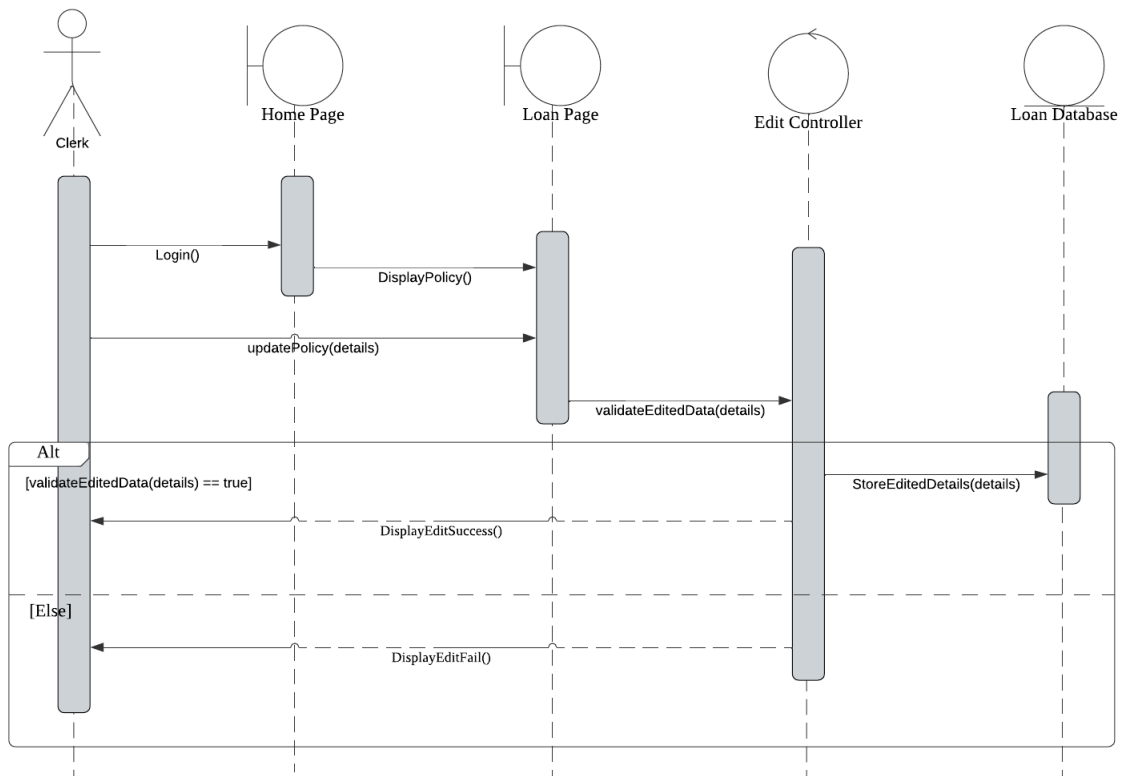
Figure 4.22: Sequence Diagram for Manage Loan Policy
