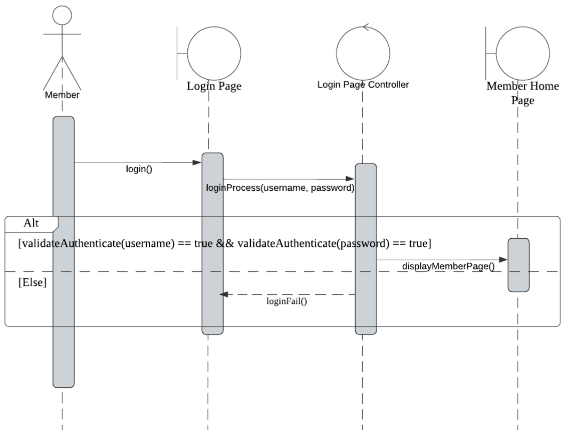
Figure 4.24: Sequence Diagram for Authentication (Member)
