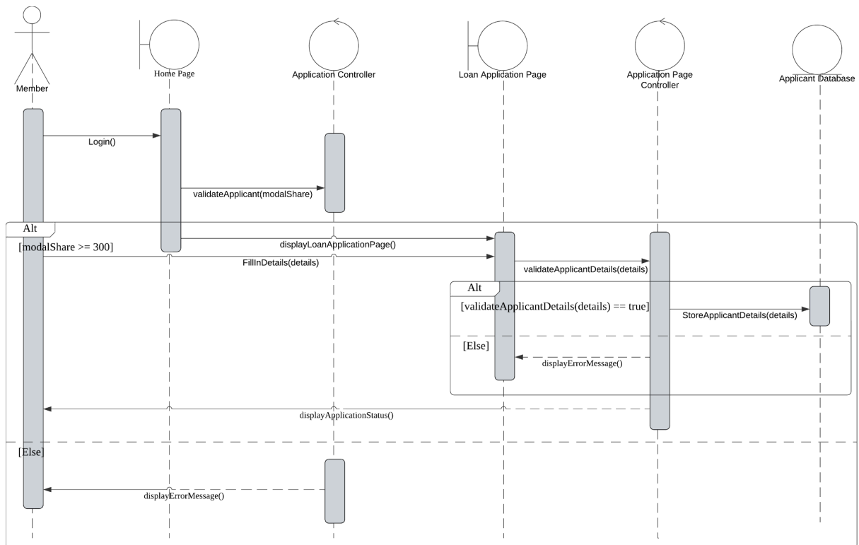
Figure 4.14: Sequence Diagram for Apply for Loan
