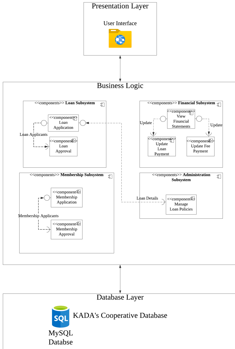
Figure 4.3: Component Diagram of KADA's Cooperative Web-Based System
