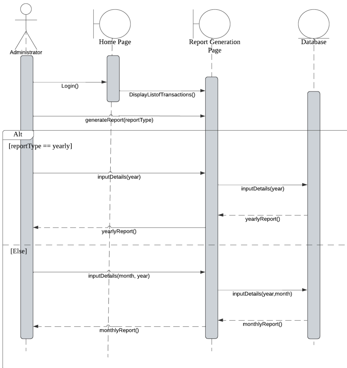
Figure 4.23: Sequence Diagram for Generate Report
