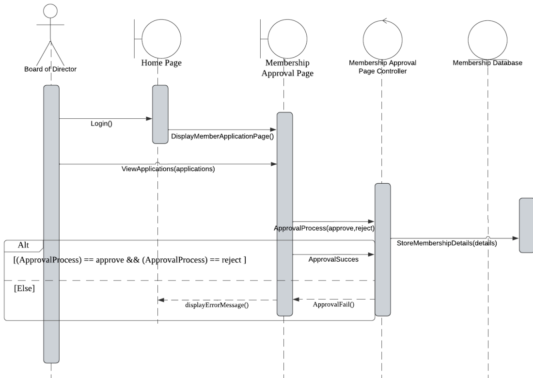
Figure 4.20: Sequence Diagram for Approve Membership Application
