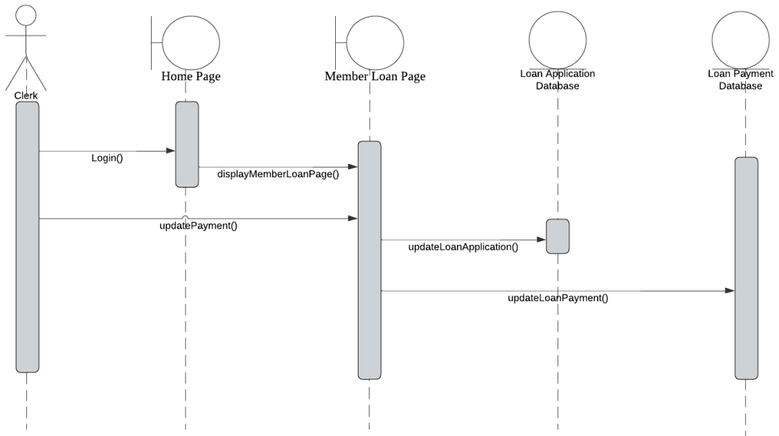
Figure 4.18: Sequence Diagram for Update Loan Payment
