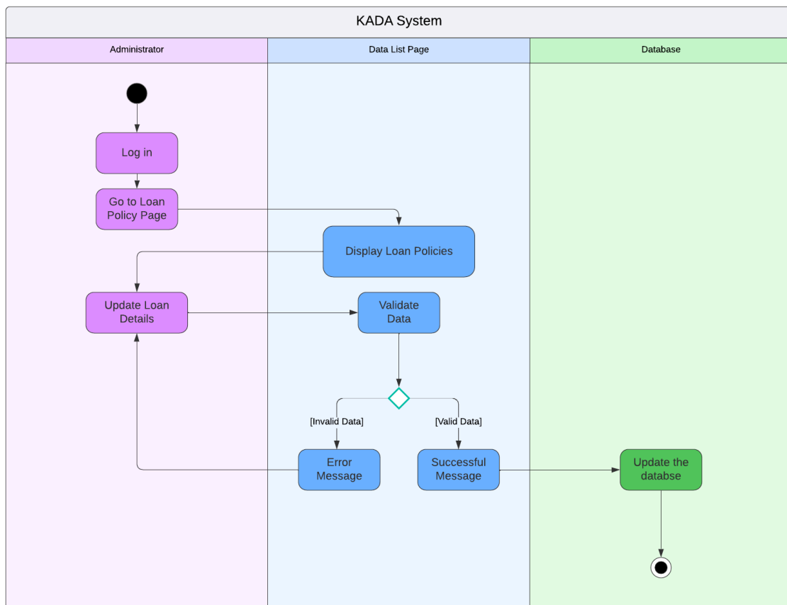
Figure 2.21: Activity Diagram for Manage Loan Policy
