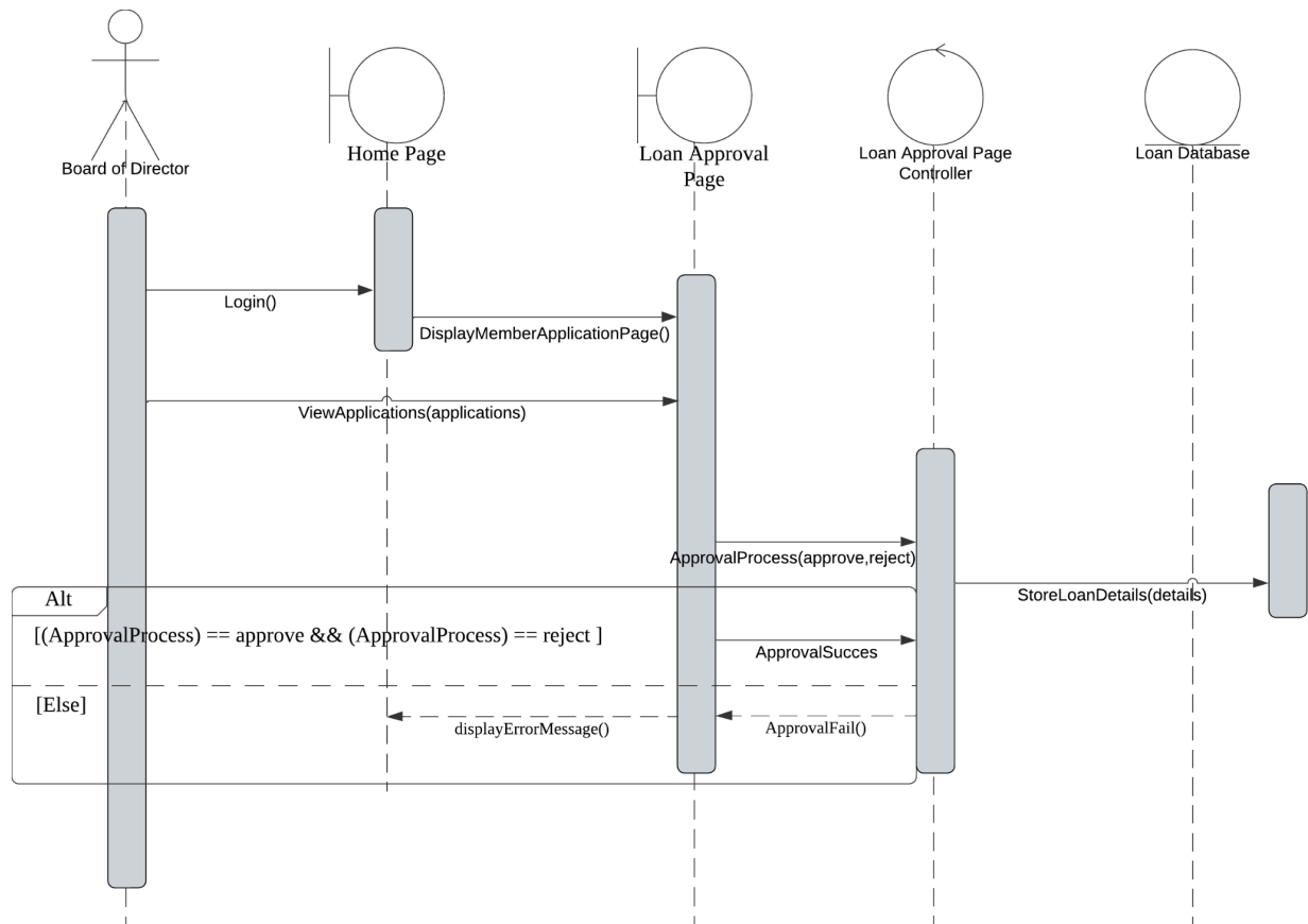
Figure 2.18: Sequence Diagram for Approve Loan Application
