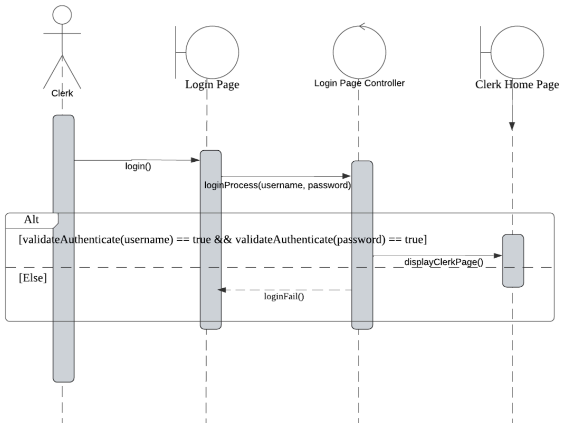
Figure 4.25: Sequence Diagram for Authentication (Clerk)
