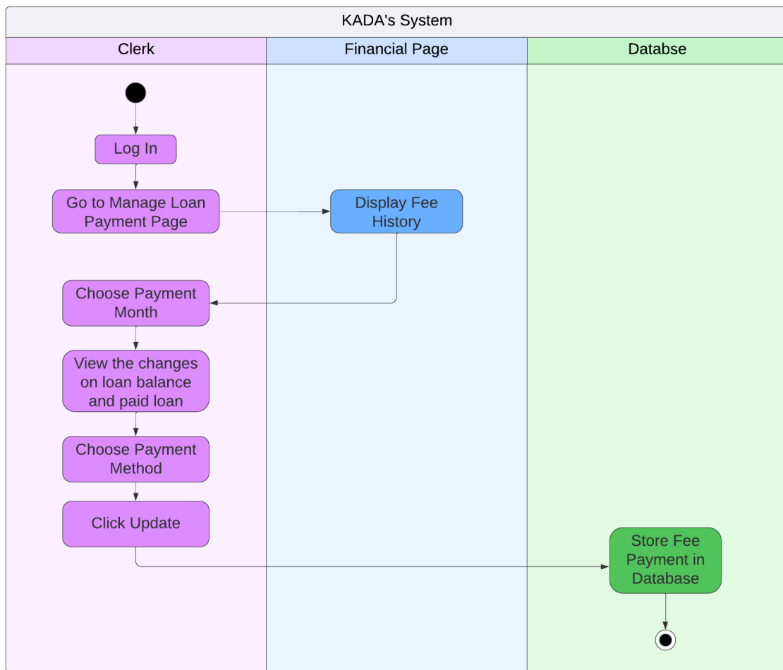
Figure 2.13: Activity Diagram for Update Loan Payment
