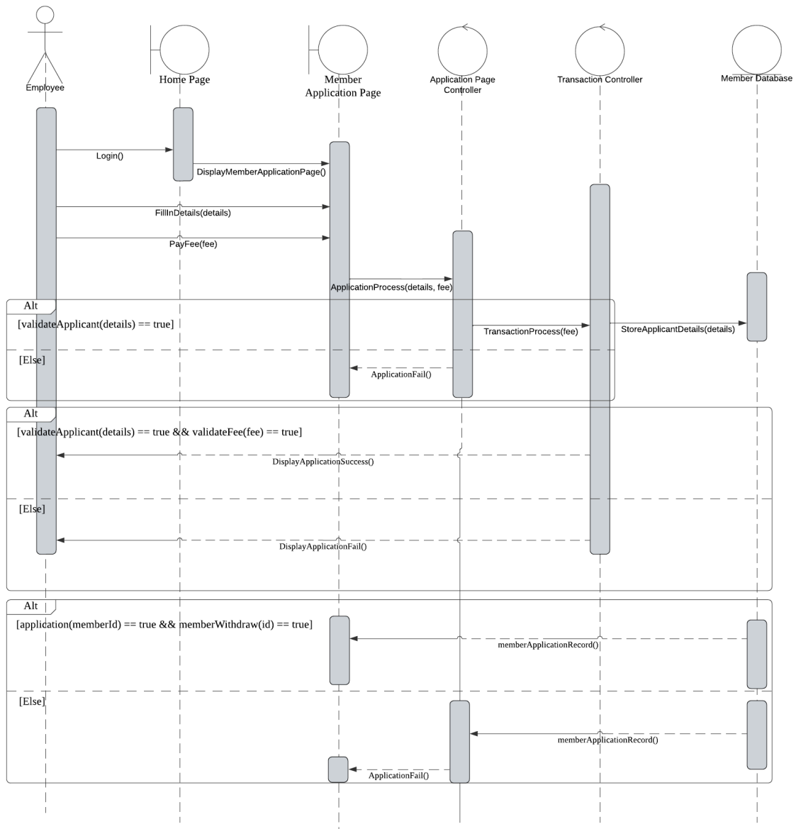
Figure 4.13: Sequence Diagram for Apply for Membership
