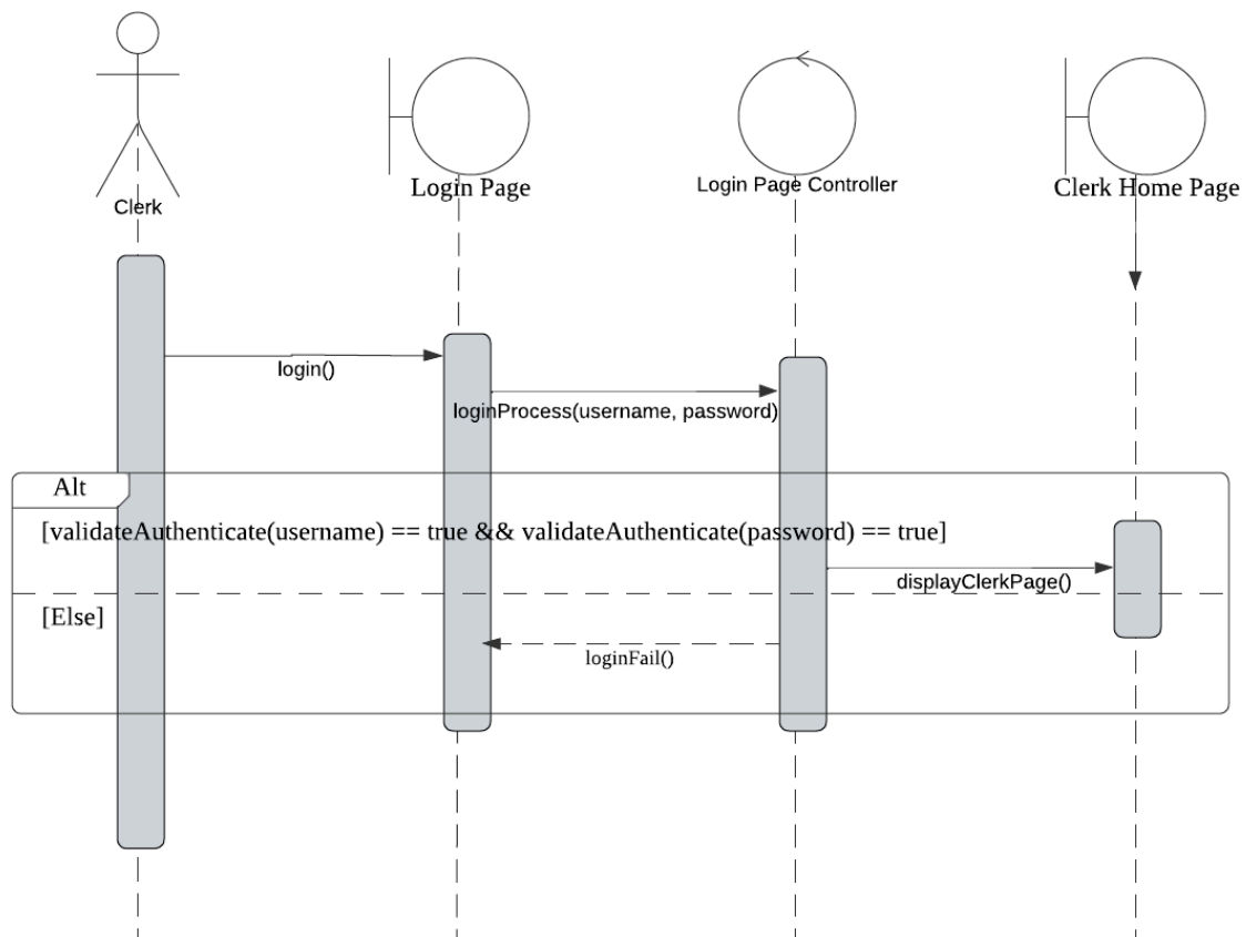
Figure 2.25: Sequence Diagram for Authentication (Clerk)
