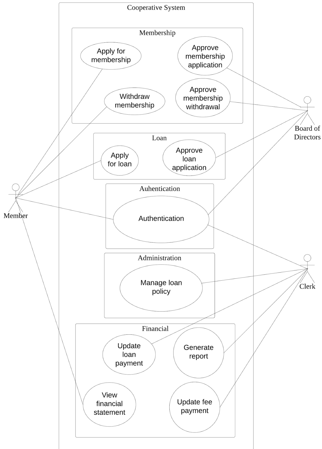
Figure 4.1: Use Case Diagram for KADA's Cooperative Web-Based System
