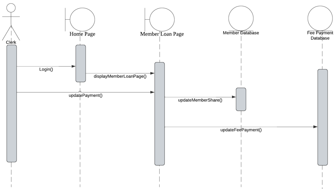
Figure 4.19: Sequence Diagram for Update Fee Payment
