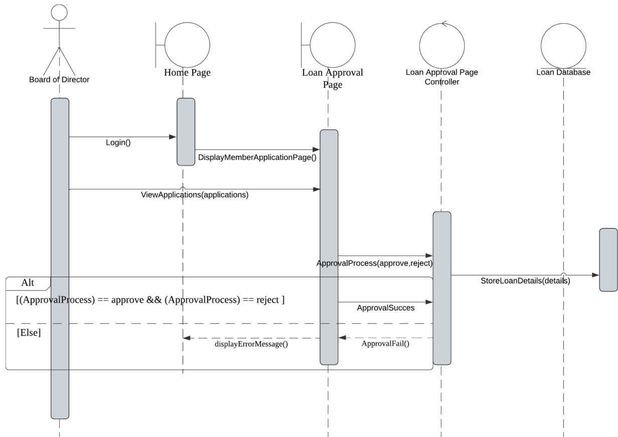
Figure 4.21: Sequence Diagram for Approve Loan Application
