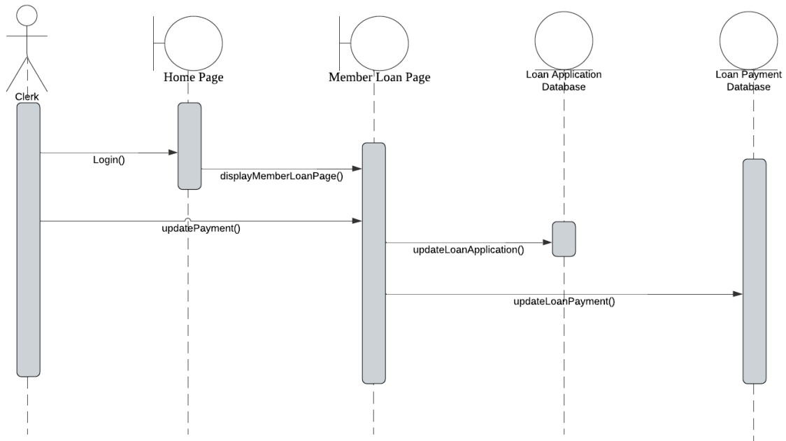
Figure 2.12: Sequence Diagram for Update Loan Payment
