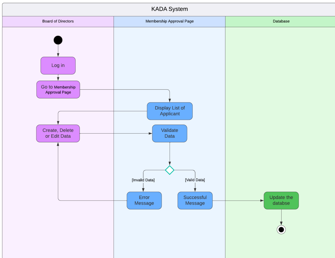
Figure 2.17: Activity Diagram for Approve Membership Application
