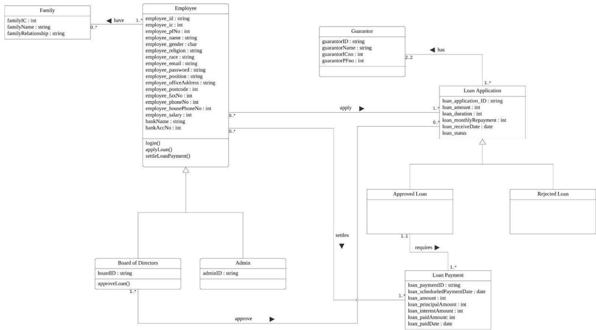
Figure 4.12 Class Diagram for Loan Subsystem
