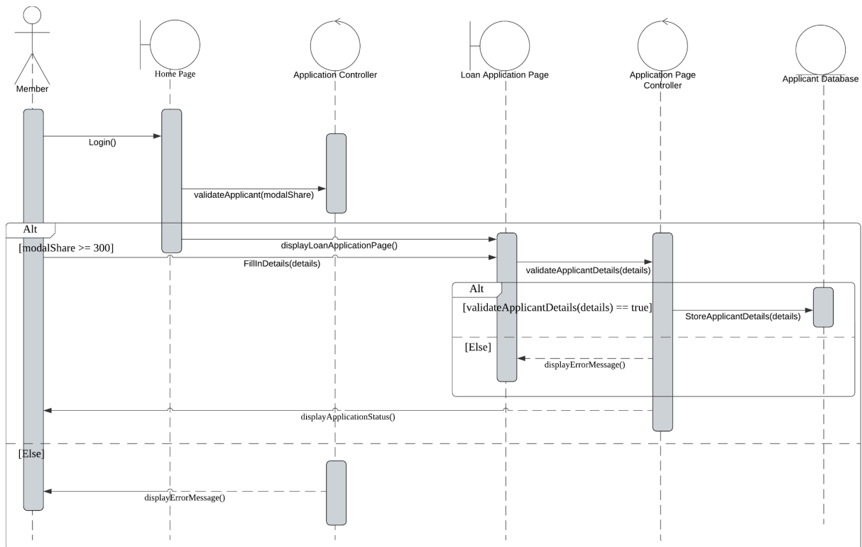
Figure 2.4: Sequence Diagram for Apply for Loan
