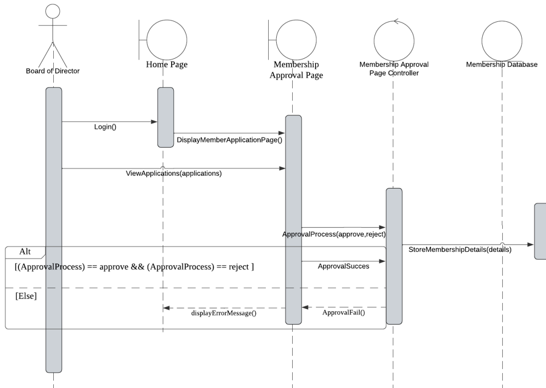
Figure 2.16: Sequence Diagram for Approve Membership Application
