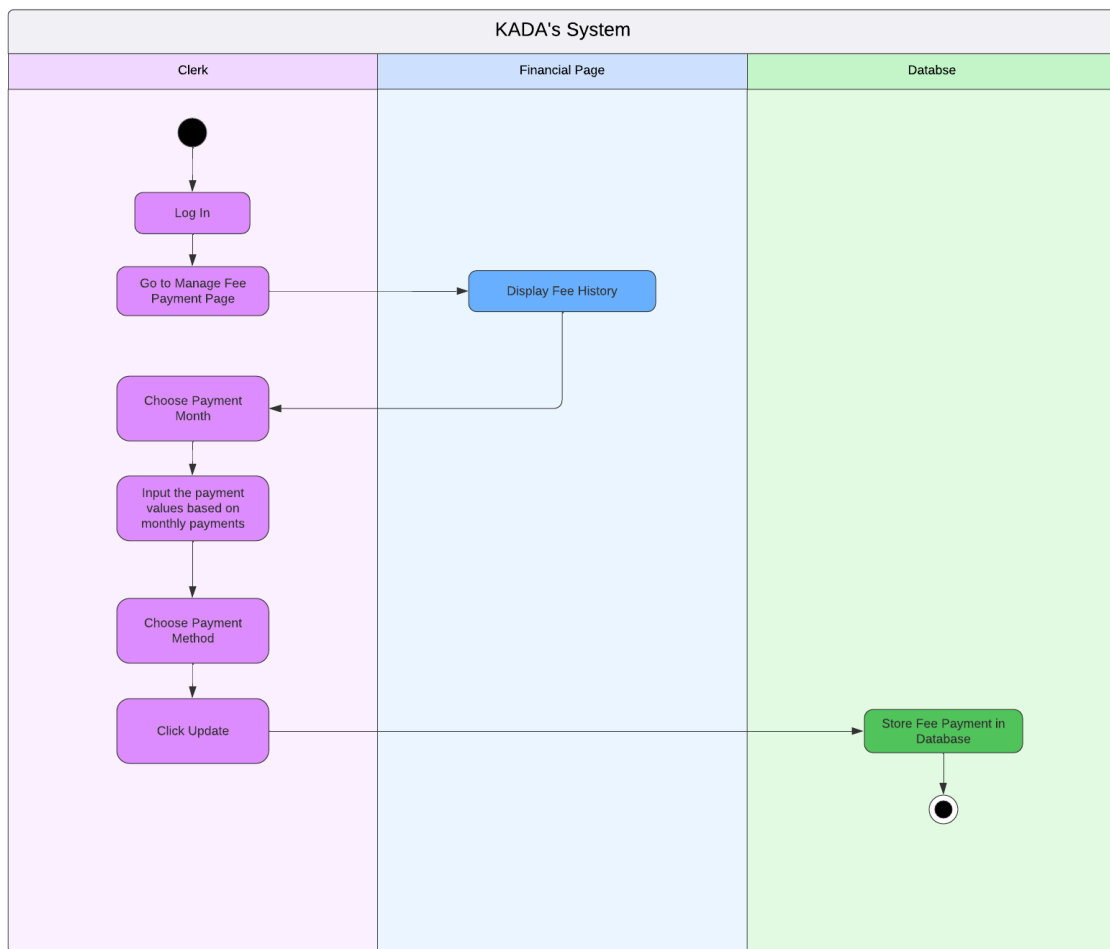
Figure 2.15: Activity Diagram for Update Fee Payment
