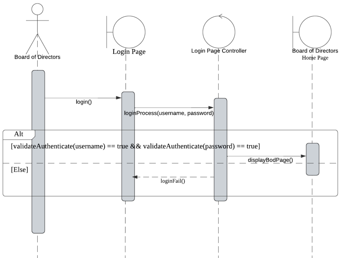
Figure 2.26: Sequence Diagram for Authentication (Board of Directors)
