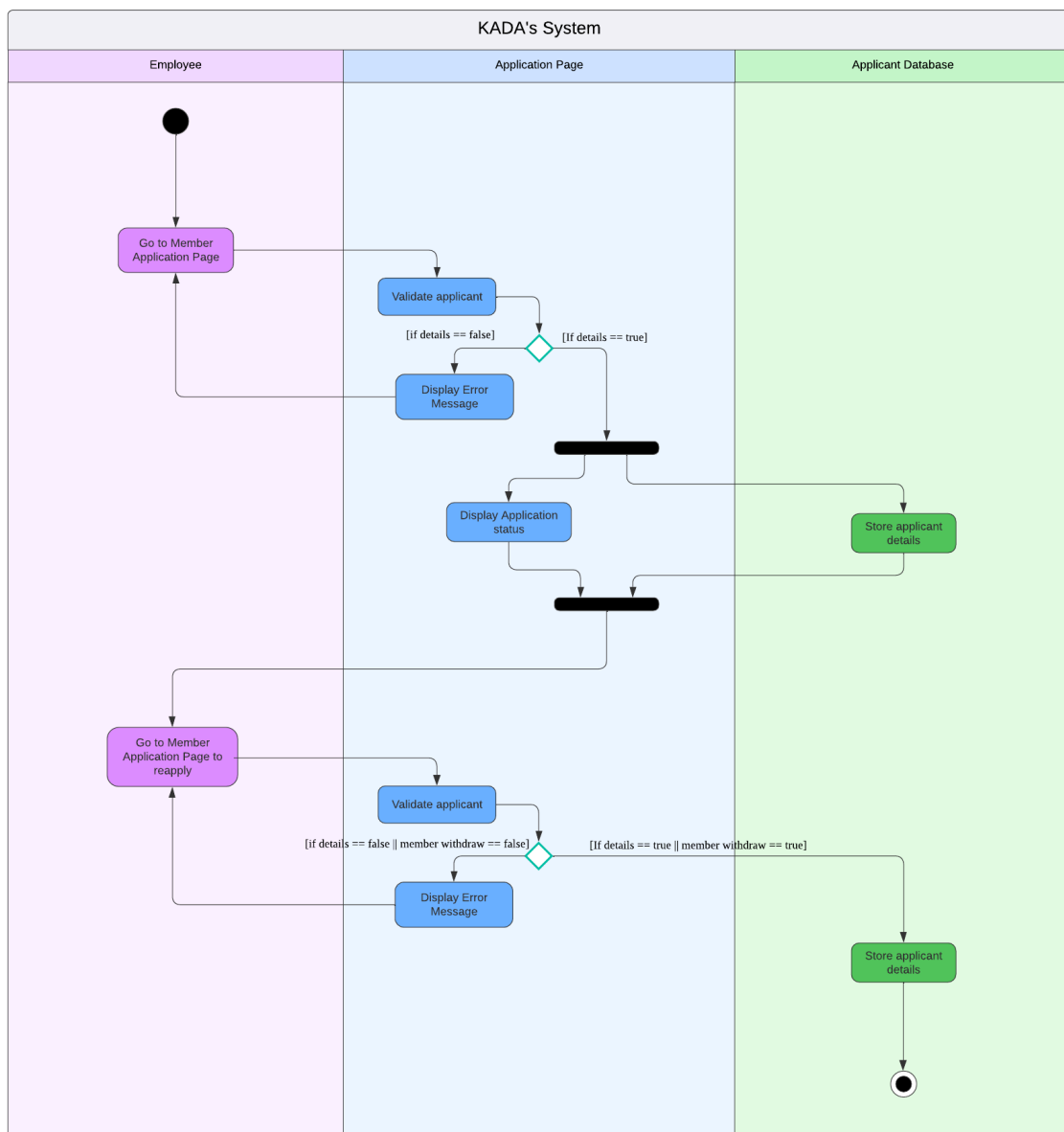
Figure 2.3: Activity Diagram for Apply for Membership
