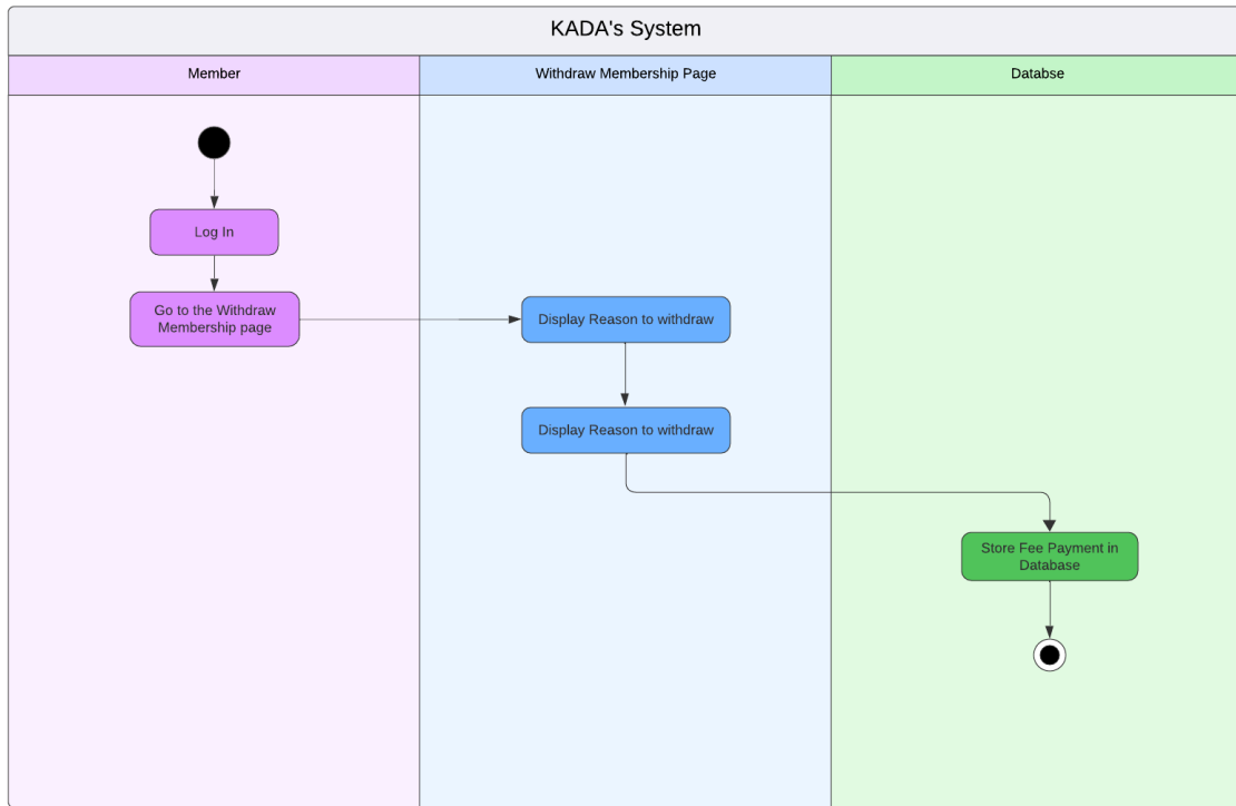
Figure 2.7: Activity Diagram for Withdraw Membership
