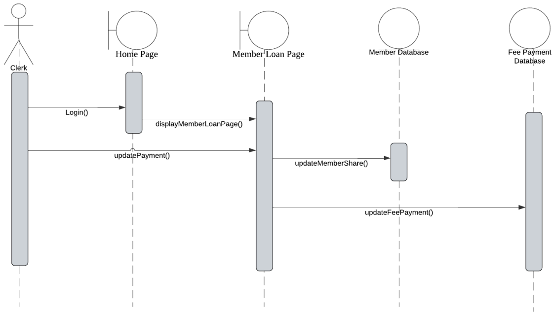
Figure 2.14: Sequence Diagram for Update Fee Payment
