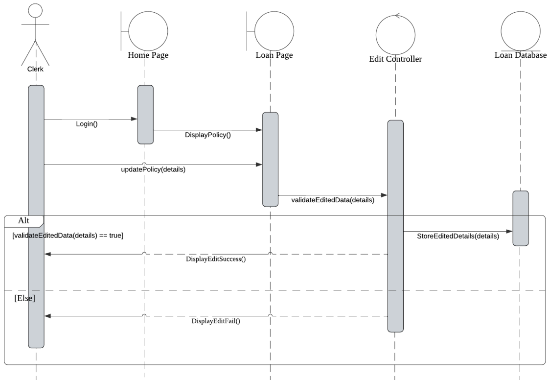
Figure 2.20: Sequence Diagram for Manage Loan Policy
